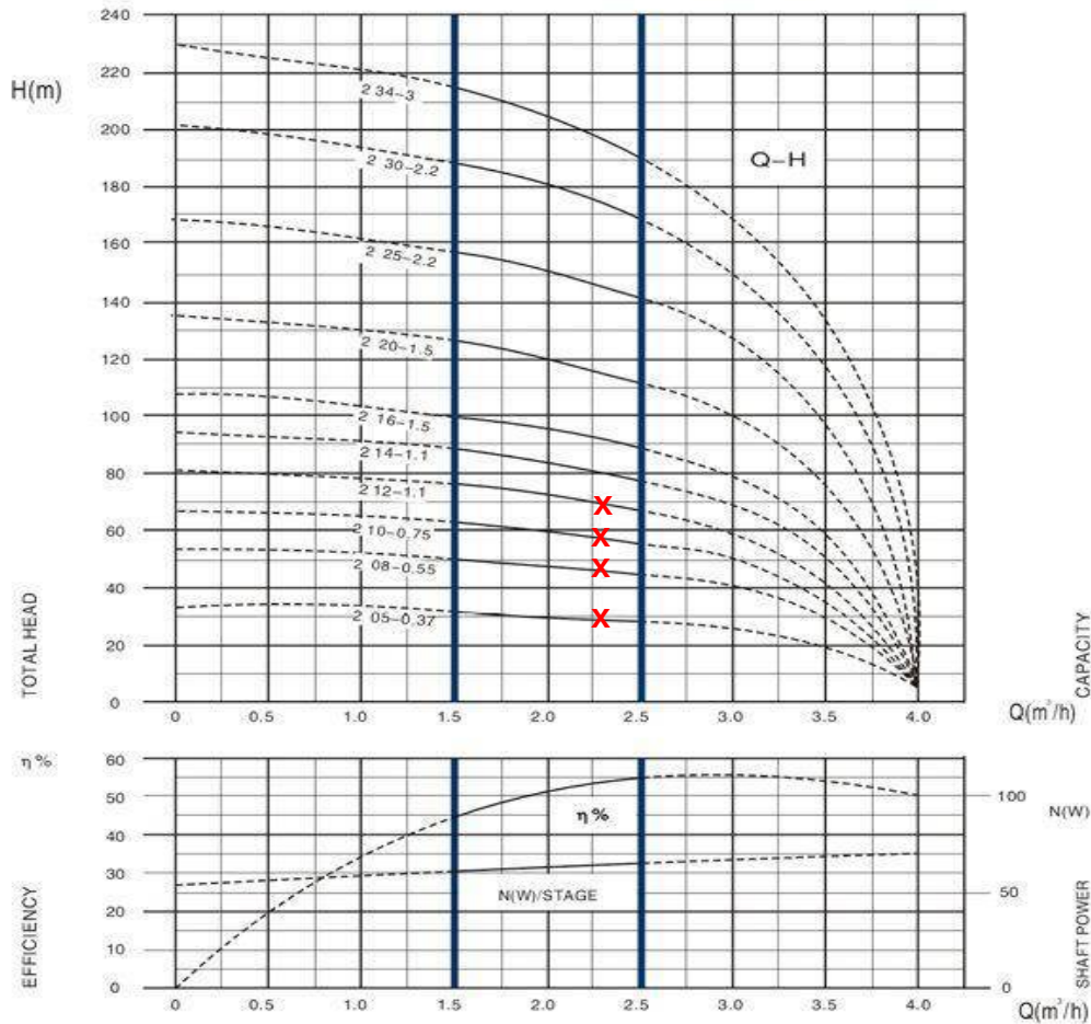
100QJ2/100QH2 SUBMERSIBLE PUMPS
